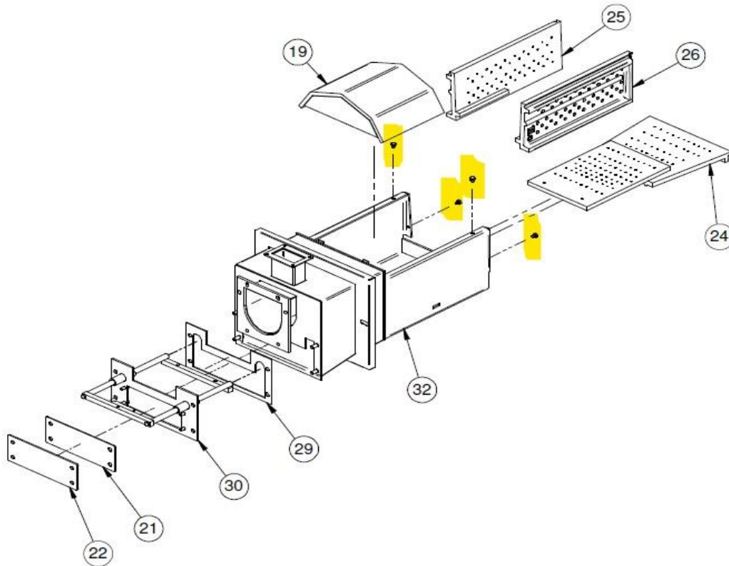
Figure 31 Burner head components 80/120 kW, moving grate
